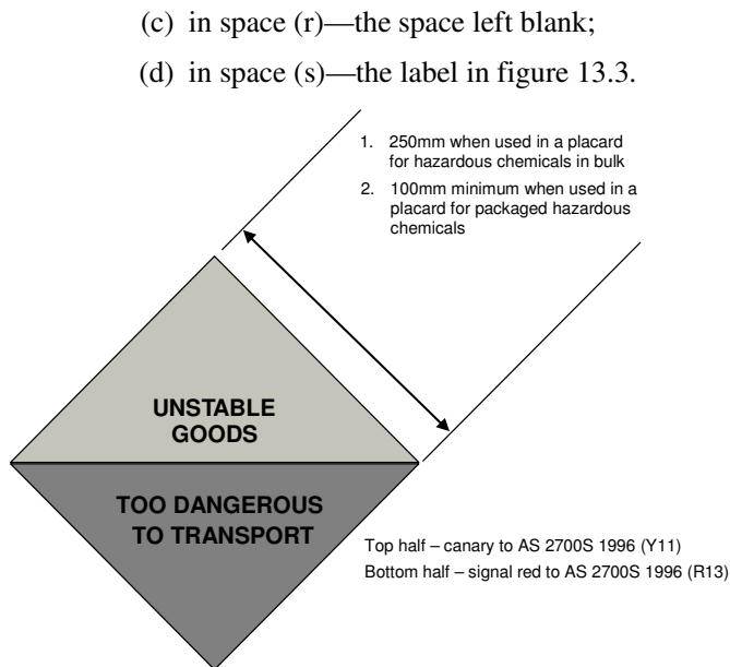
Figure 13.3 Label for unstable explosive, organic peroxide type A or self-reactive substance type A
